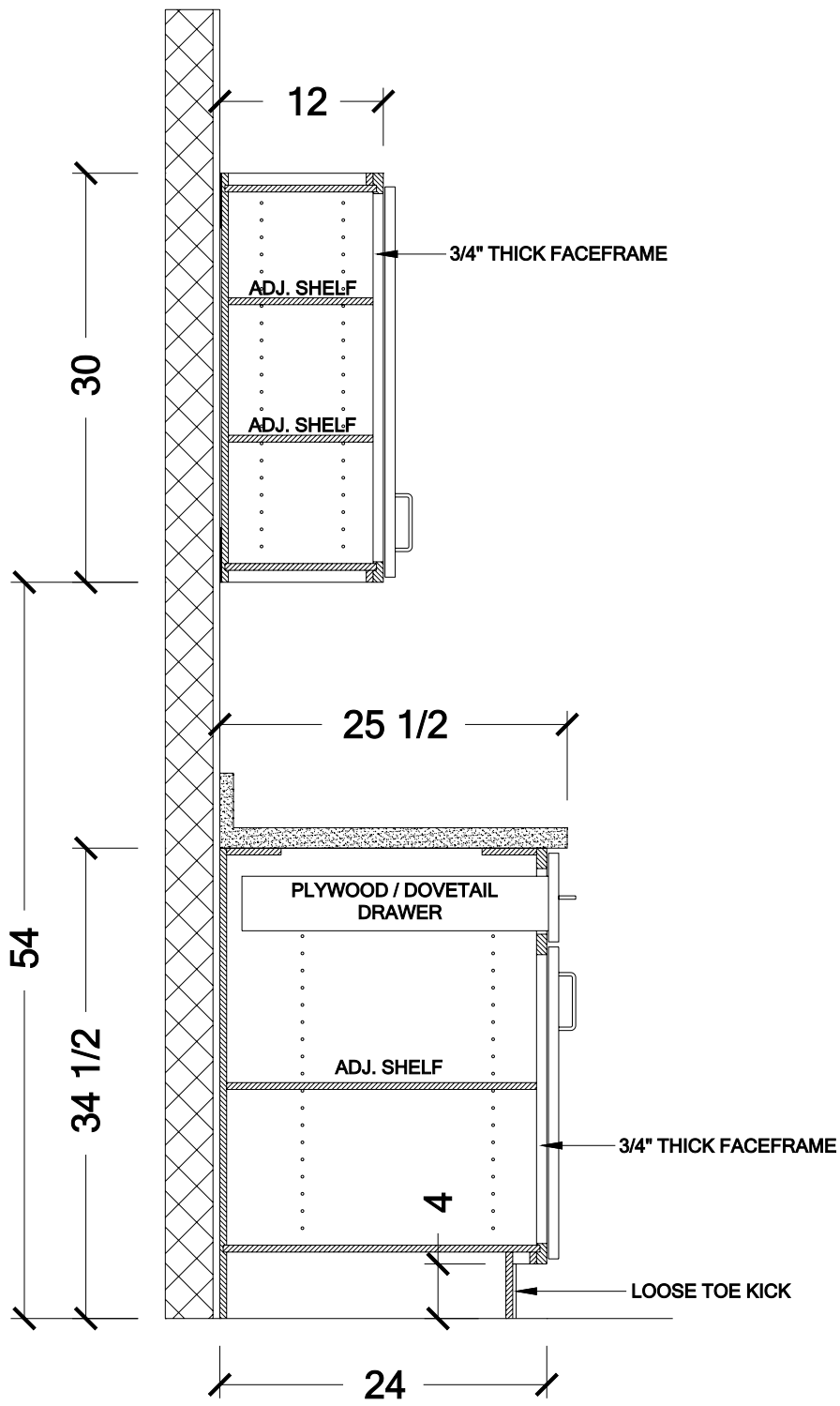
TYPICAL WOOD CABINET SECTION VIEW
